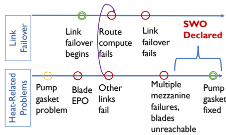
Fig. 1: Network recovery-sequence cluster showing relationship between failure and recovery events
