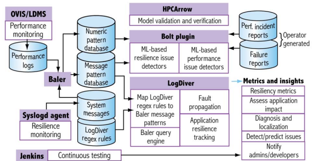
Fig. 4: HMDSA Infrastructure. Data sources (left); analysis results and responses (right). HMDSA will enhance our capabilities for advanced automated analyses of failure and performance degradation EoI and to inform system-level and application-level responses.
