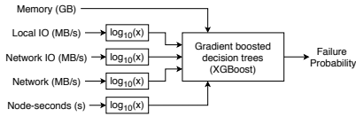
Fig. 7: ML model for predicting impending failure of a job.
