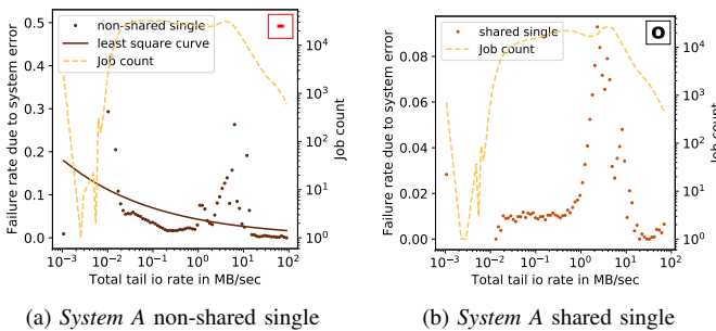
Fig. 4: Failure rate vs total tail local IO rates
