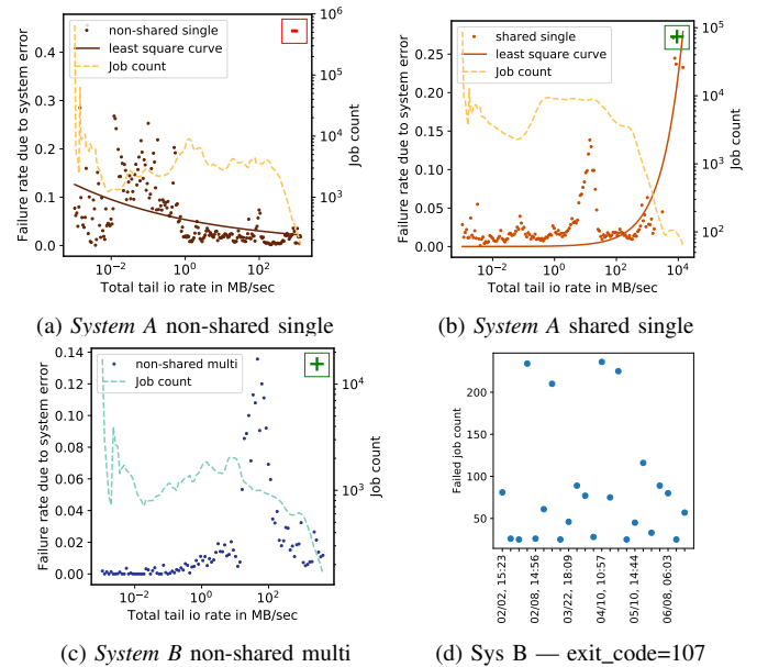
Fig. 5: Failure rate vs total tail network file system I/O rates
