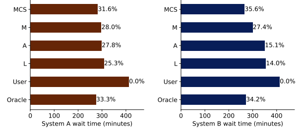
Fig. 11: Overall Job Wait time for System A and System B using different runtime predictors. The values over the bars show improvements over user estimated runtime
