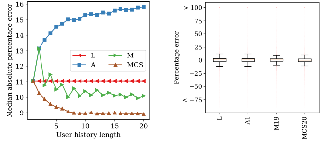
(a) Different models performance with different history lengths on the test set with best training set (b) Percentage error distribution for different models on test set with best history length as per training set.
