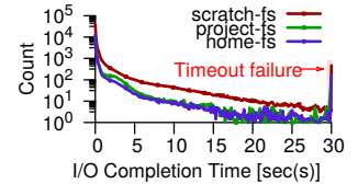
Figure 5: Wrex measured latency on three file partitions.
